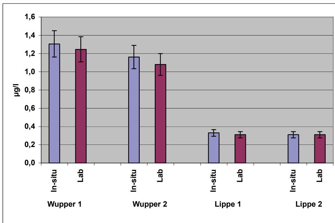
Fig. 3.3.-1: Influence of delayed acidification (in-situ/arrival at laboratory) on lead concentrations of original sample. Average value of repeat determinations (µg/l) and range of extended measuring uncertainty (U).
