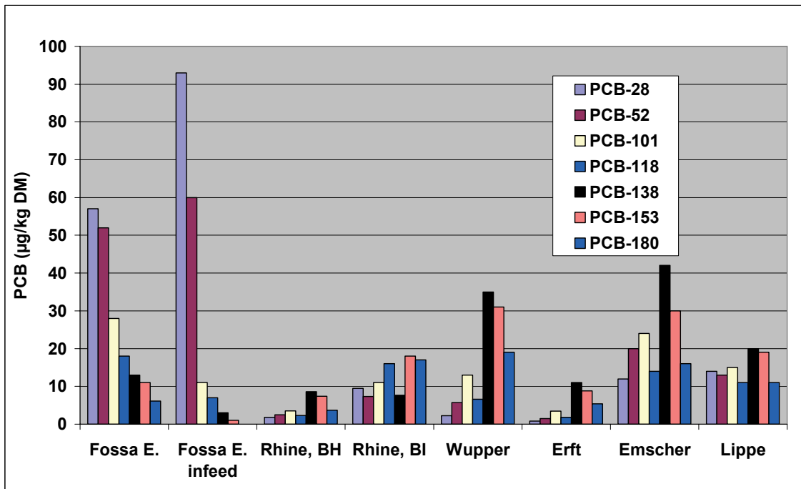
Fig. 4.2.1-1: PCB samples of suspended matter obtained from six monitoring stations versus two monitoring stations at the Fossa Eugenia influenced by mining. DM = dry mass
