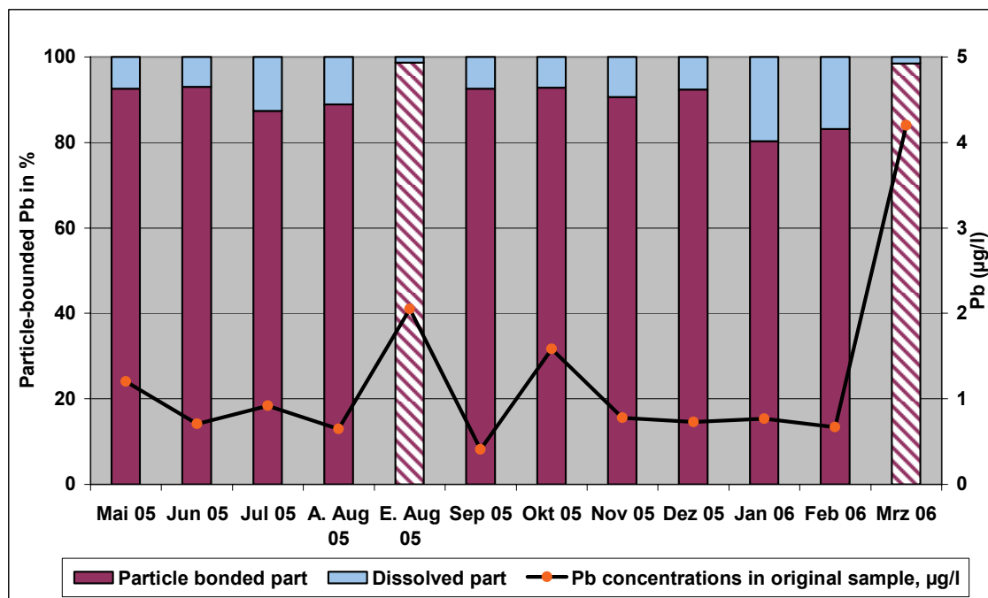
Fig. 4.1.3-2 : Distribution of lead contents over dissolved and particulate phases over time versus concentrations in the original sample in Bad Honnef (Rhine).
