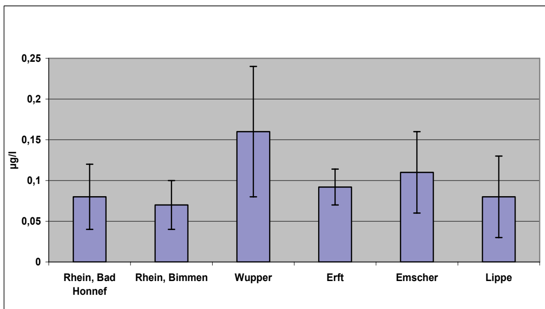
Fig. 4.1.2-11: Lead in filtered sample. Average values and standard deviation of concentration at all monitoring stations
