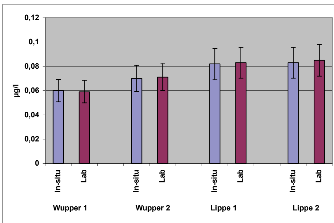
Fig. 3.3.-2: Influence of delayed acidification (in-situ/arrival at laboratory) on cadmium concentrations of original sample. Average value of repeat determinations (µg/l) and range of extended measuring uncertainty (U).
